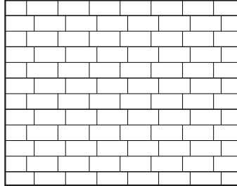
RUNNING QUARTER BOND
